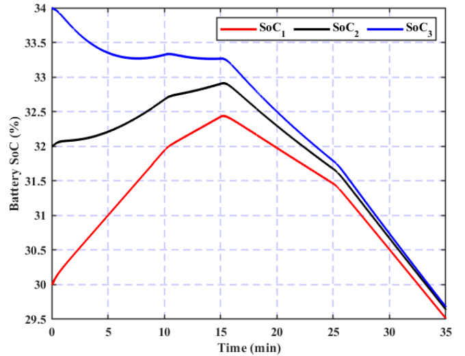
Fig. 8: Batteries' state of charge. The proposed controller successfully balances the SoCs, reducing the initial 4% spread and maintaining all units within a safe operating range while preventing over-charging and over-discharging
